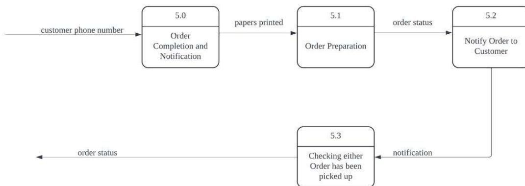
c) Child diagram
